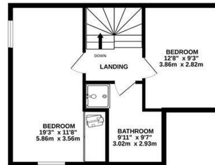
2ND FLOOR 442 sq.ft. (41.1 sq.m.) approx.
